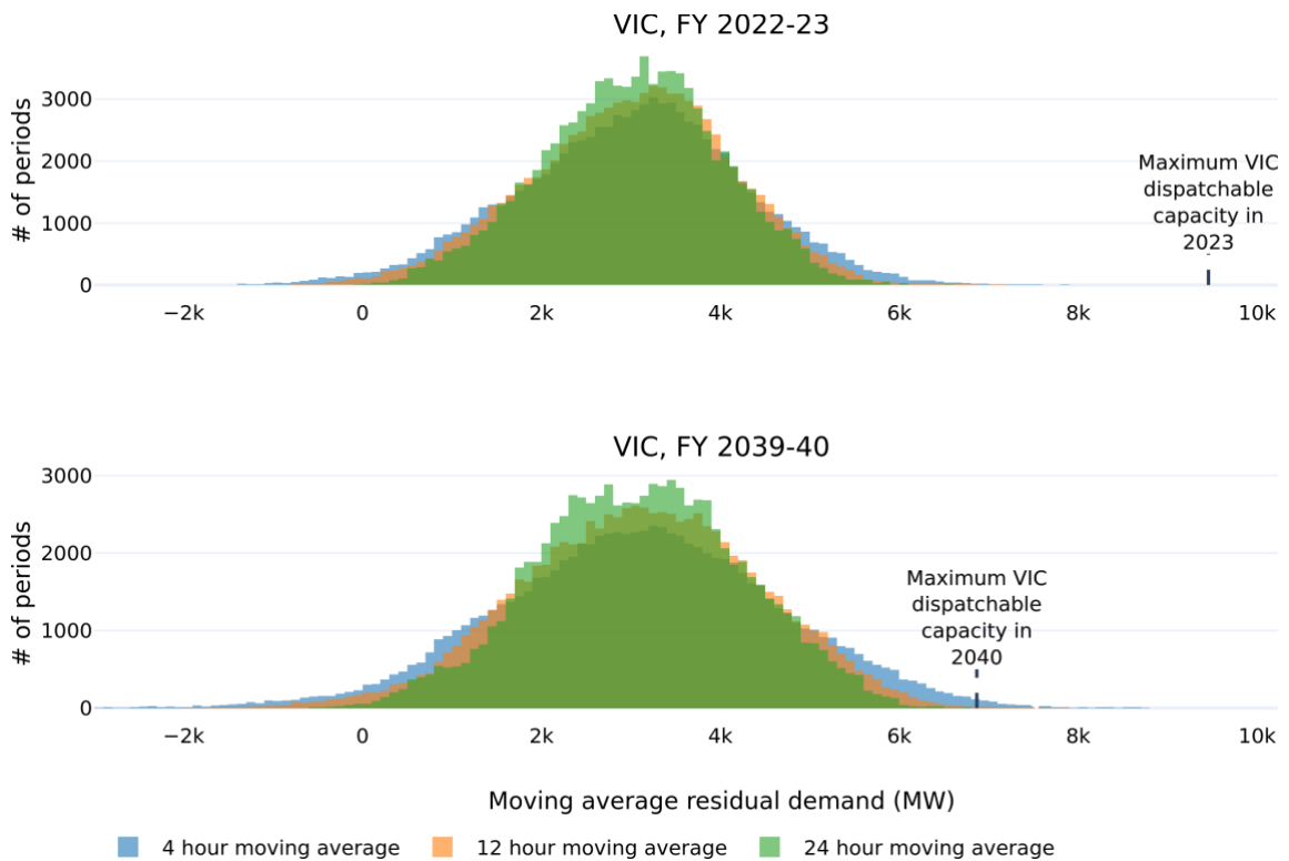
Figure 17. Histogram of rolling average Residual Demand in Victoria in 2022/23 and 2039/40
