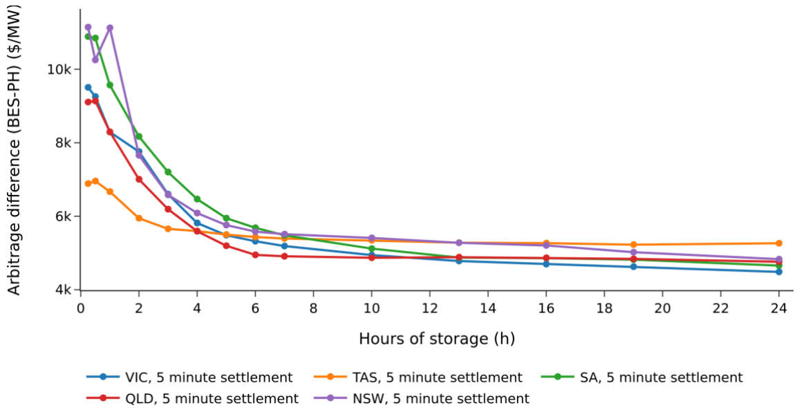
Figure 36. Difference between battery storage and PH Arbitrage Revenue
