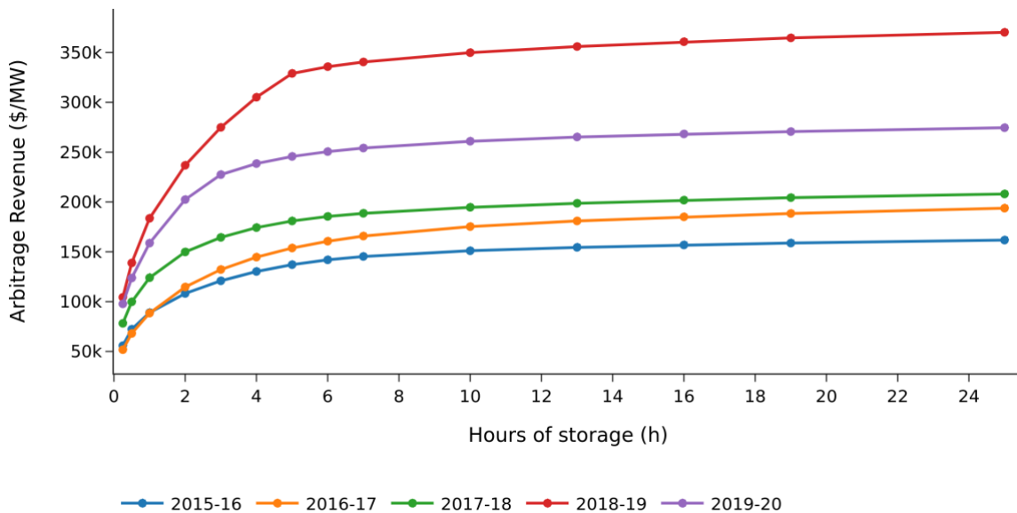
Figure 16. Arbitrage revenue as a function of storage duration in Victoria from 2015/16 to 2019/20
