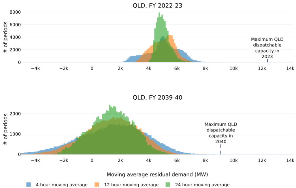
Figure 31. Histograms of Queensland Residual Demand
