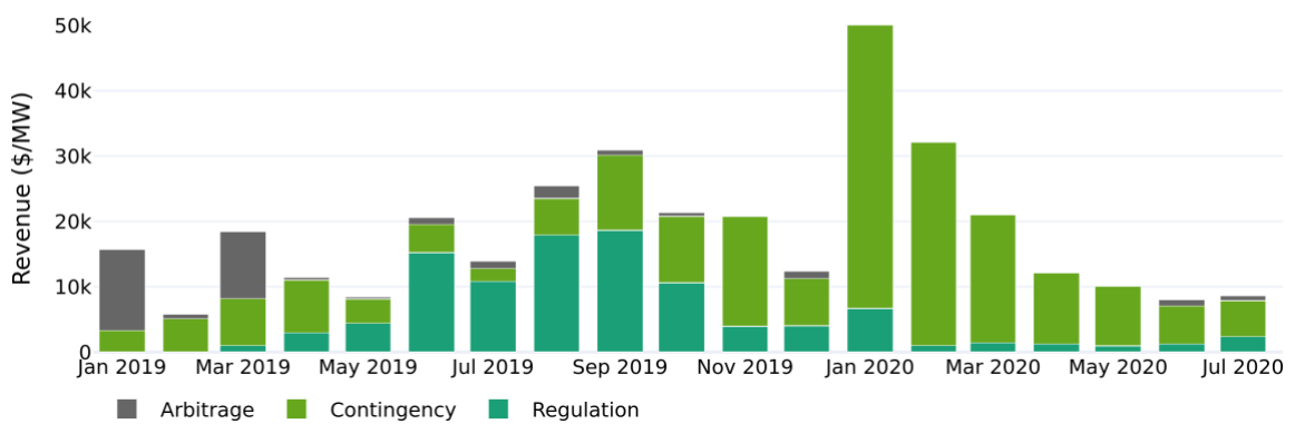
Figure 26. Dalrymple North Battery Energy Storage System FCAS revenue
