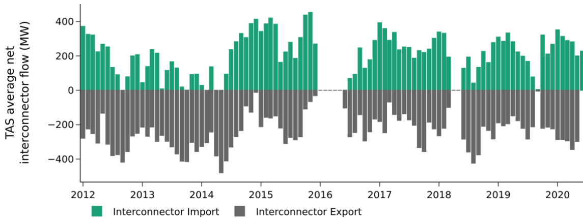
Figure 8. Tasmania monthly average interconnector flows 2012 to 2020 (negative is export from TAS)
