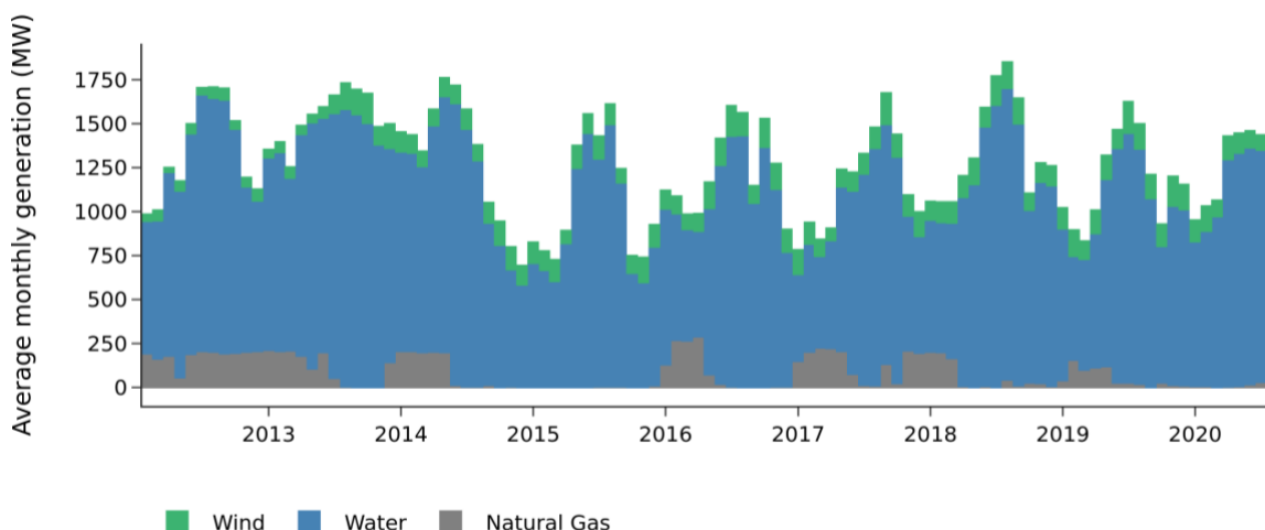
Figure 3. Tasmania monthly average grid-based supply 2012 to 2020
