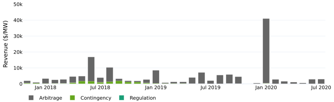
Figure 25. Ballarat Battery Energy Storage System FCAS revenue
