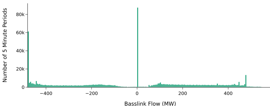
Figure 12. Basslink power flow histogram (July 2014 to June 2020)
