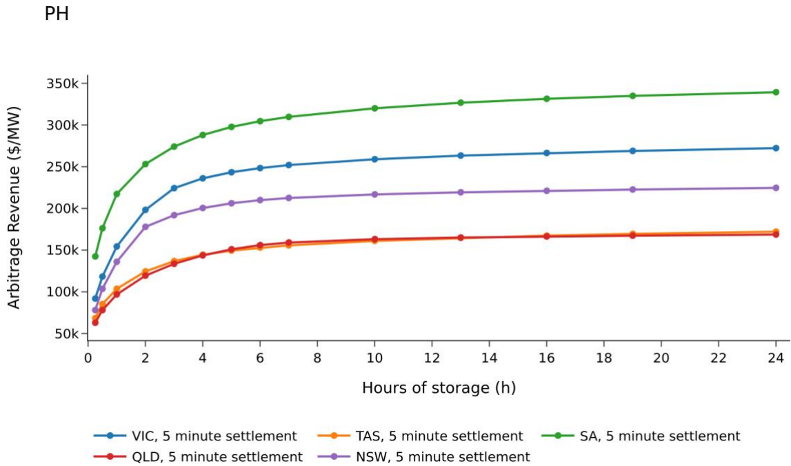
Figure 34. Pumped hydro Arbitrage Revenue
