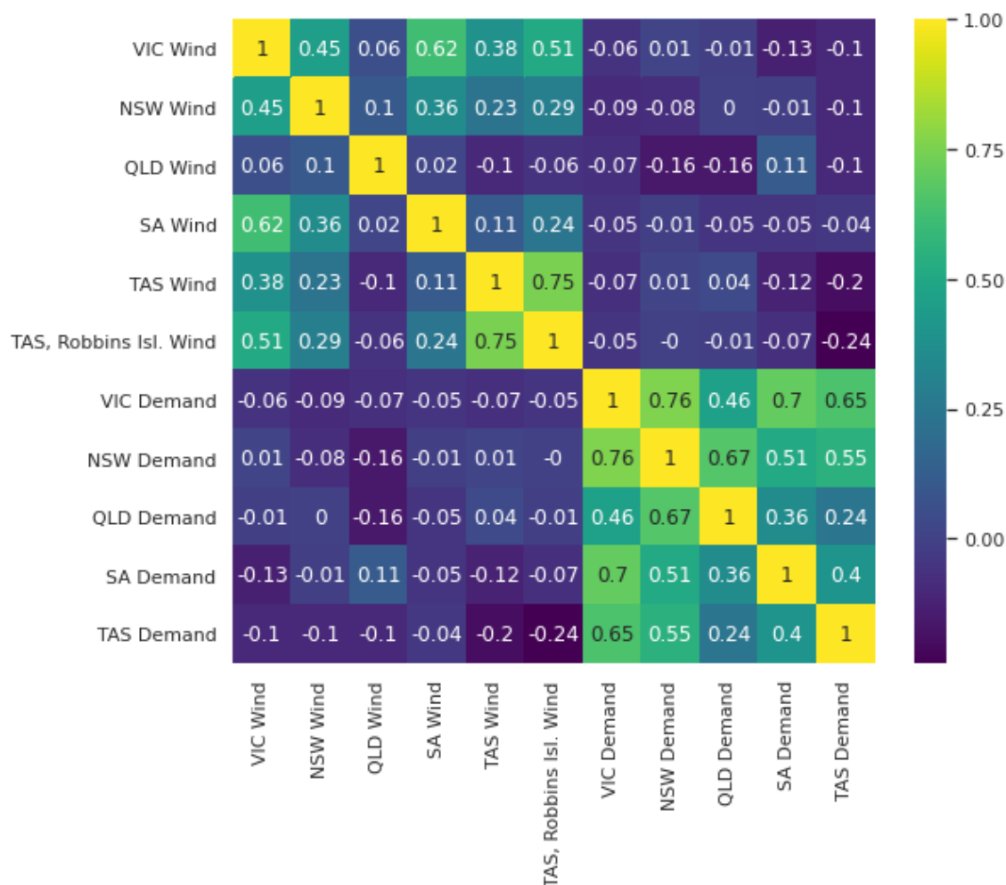
Figure 13. All regional wind and demand correlation matrix
