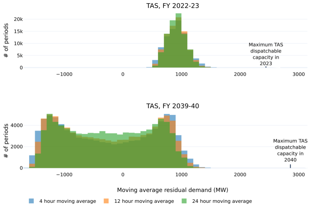
Figure 33. Histograms of Tasmanian Residual Demand
