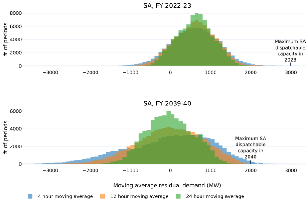
Figure 32. Histograms of South Australian Residual Demand
