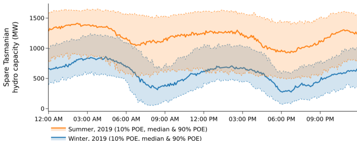
Figure 9. Spare Tasmanian hydro capacity for summer and winter in 2019 calendar year.
