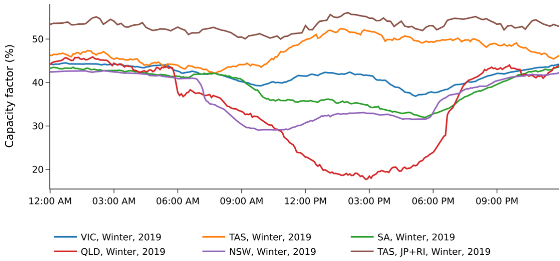
Figure 15. Average winter regional wind capacity factors measured through the day
