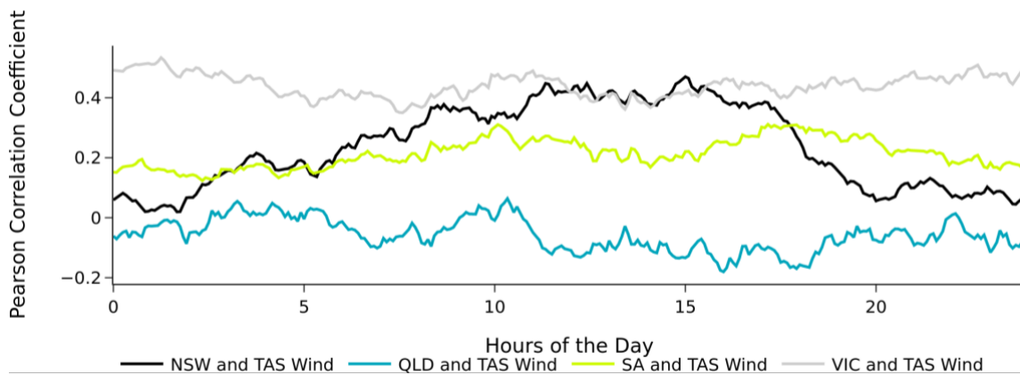
Figure 40. Autumn Pearson R correlation coefficient
