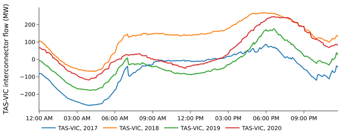
Figure 11. Basslink interconnector flow, (positive value is export from TAS)
