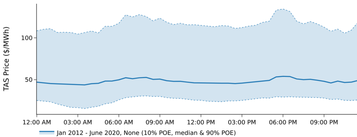
Figure 7. Eight-year average Tasmanian Price throughout the day
