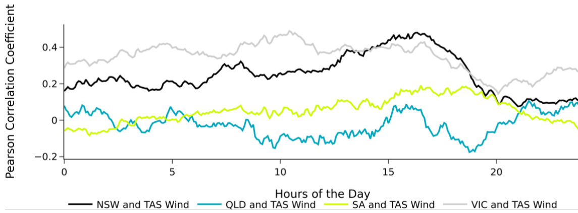
Figure 42. Spring Pearson R correlation coefficient
