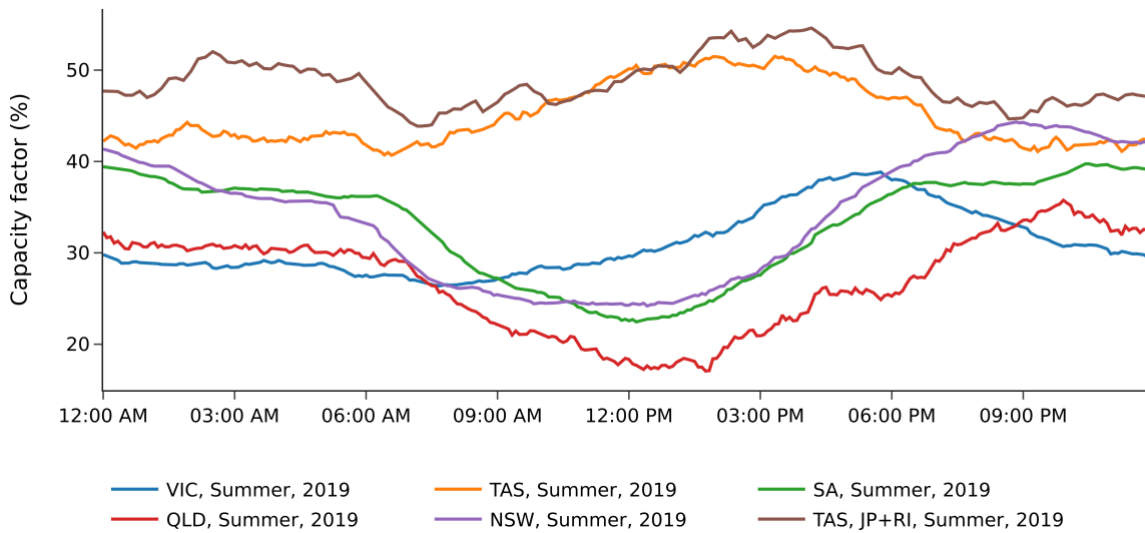
Figure 14. Average summer regional wind capacity factors measured through the day
